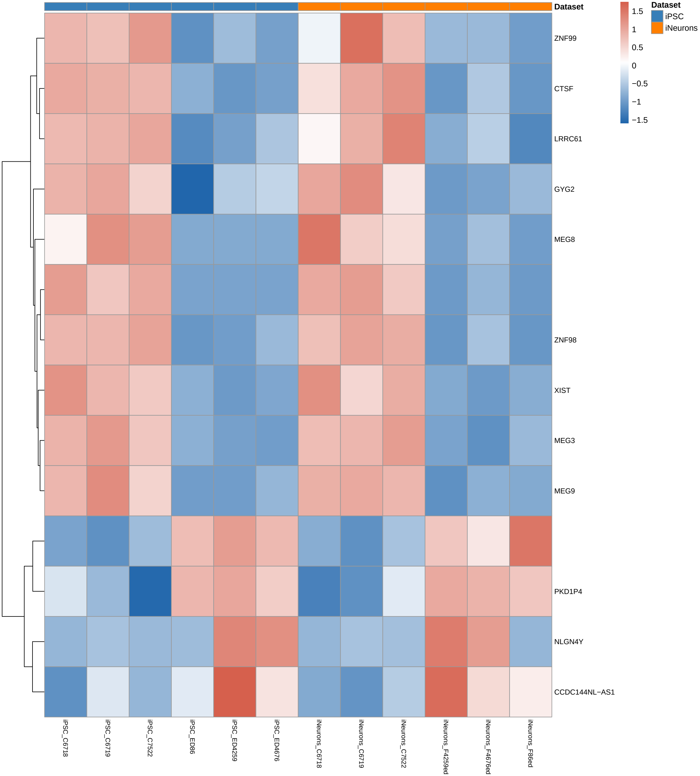
Shared DEGs (z-scored VST) control_vs_FA_edited | iPSC || iNeurons
